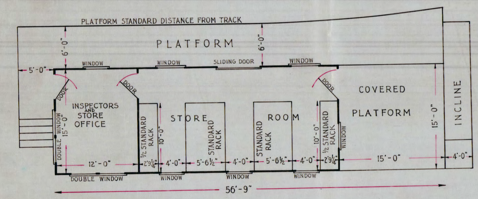
PLAN OF STORE BUILDING SCALE: 1/8" = 1'
