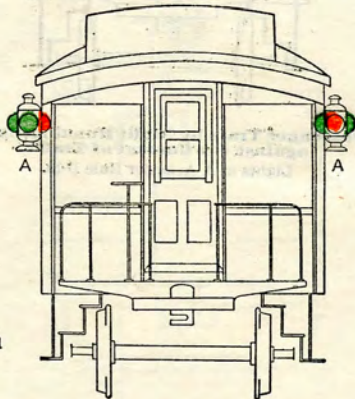
Rear of Passenger Train by Night Running with the Current of Traffic on a Slow Speed Track.
