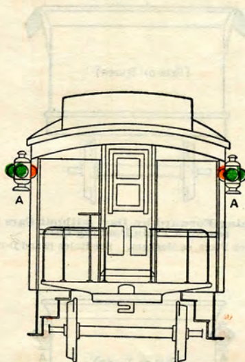
Rear of Passenger Train by Night when on Siding to be Met or Passed by Another Train. Lights at A A, as Markers, showing Green toward Engine, side and to rear. See Rules 19 and D-19.
