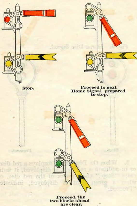
Fig. 4. Home and Distant Semaphore Signal.
