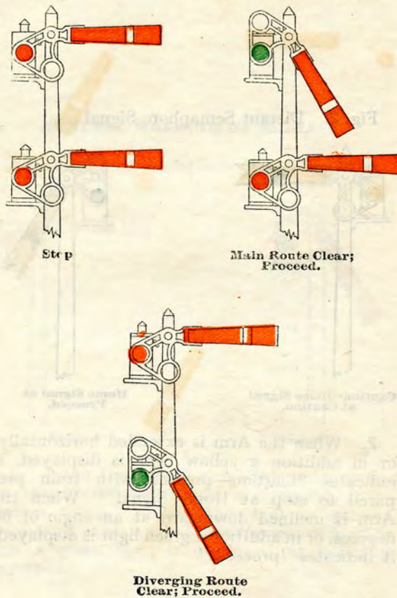
Fig. 3. Two Arm Home Semaphore Signal.
