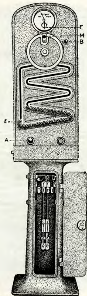
Fig 1. ELECTRIC HIGH SPEED TRAIN STAFF—MODEL No. 2. Front View of Instrument with all staffs in.
