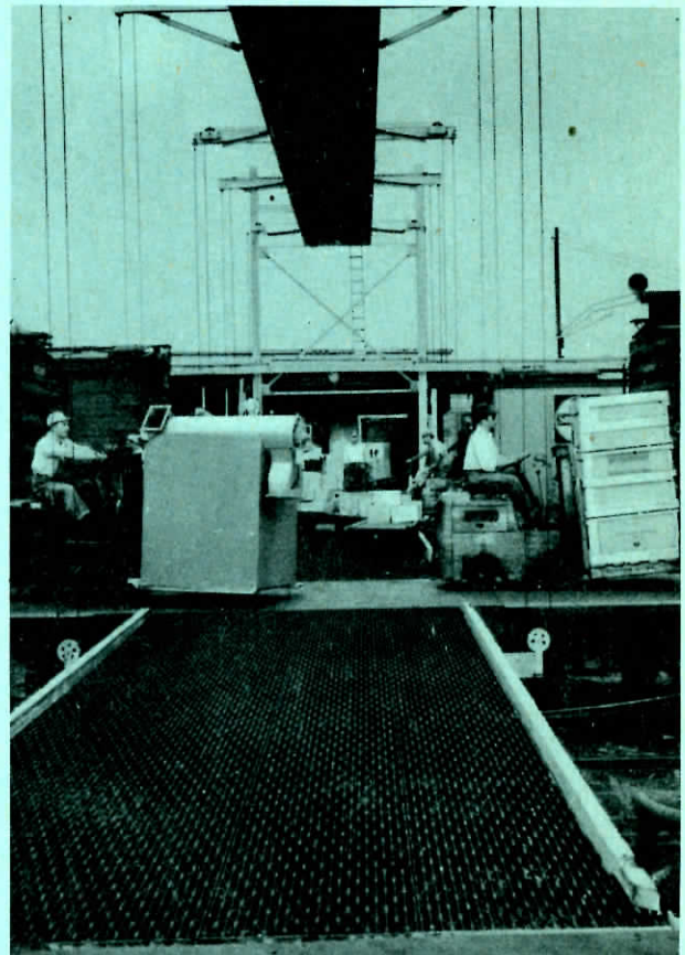
Special drop bridges between platforms and modern equipment speeds the loading and unloading of LCL shipments at important Santa Fe freight stations.
